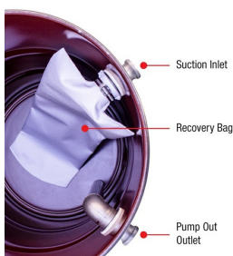
AV1-55 Top View Inside of Drum
