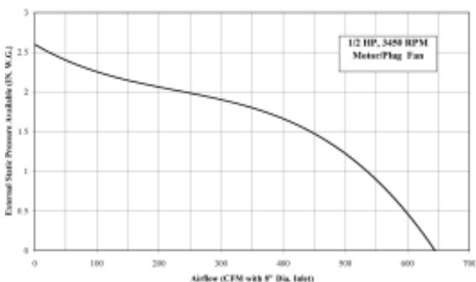
Model SM-5 UNIT PERFORMANCE CURVE at 60 Hz (250 wheel)
