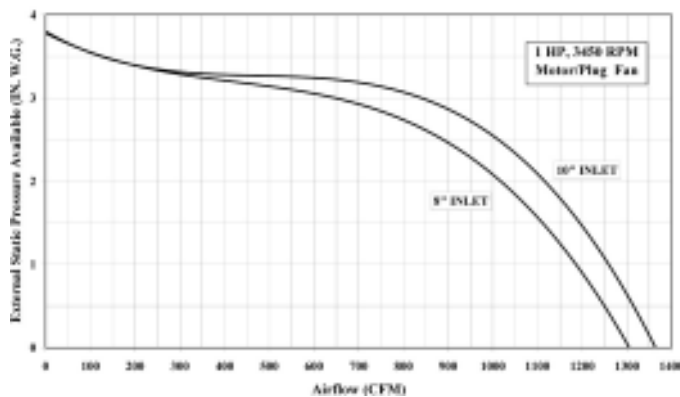
Model SM-5 UNIT PERFORMANCE CURVE at 60 Hz (250 wheel)
