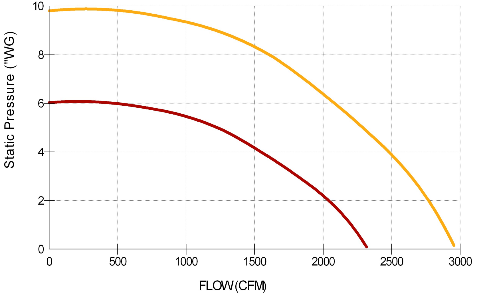
TEK280 at Required RPM 3450 and Max RPM 4400
