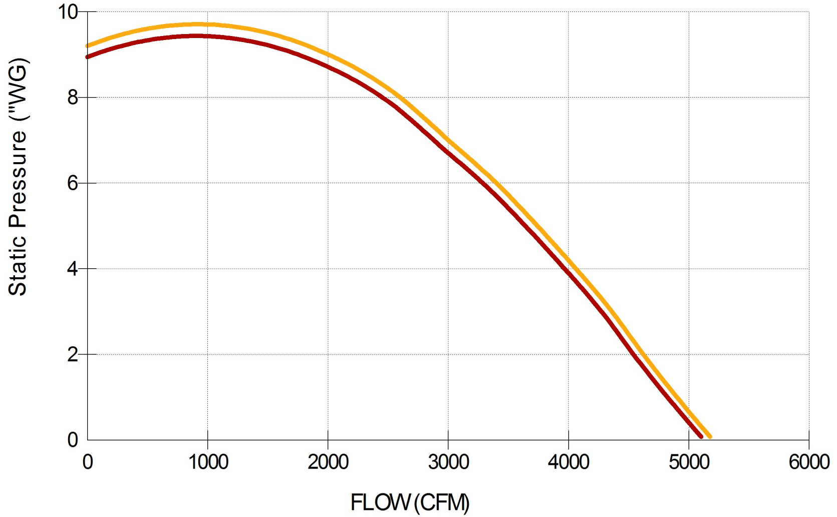
TEK355 at Required RPM 3450 and Max RPM 3500
