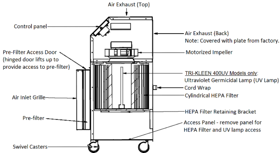
TRI-KLEEN 400 Series - side view showing internal components
